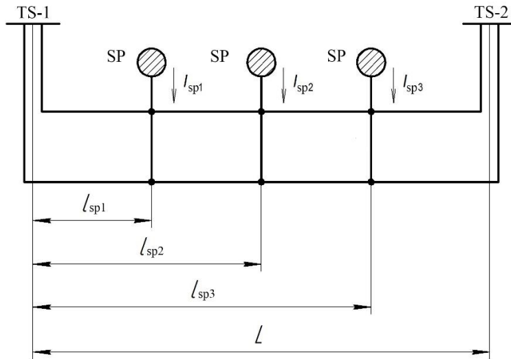
Fig. 1. Block diagram of the traction power supply network with three supply points: TS-1, TS-2 – traction substations; I_{sp1} , I_{sp2} , I_{sp3} – currents of three supply points; L – length between traction substations
