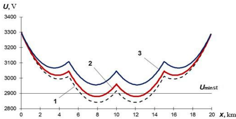
Fig. 3. The value of the voltage at pantograph at a voltage on the bus TS 3300 V:
