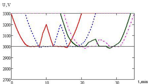
Fig. 6. Graphs voltage at the intellectual TPSS
