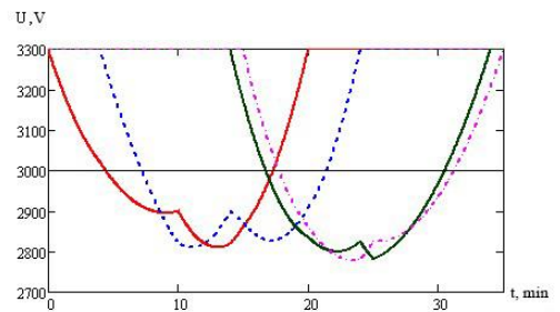
Fig. 7. Graphs voltage at the usual TPSS
