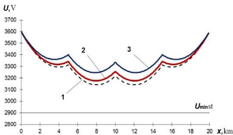
Fig. 4. The value of the voltage at pantograph at a voltage on the bus TS 3600 V:
