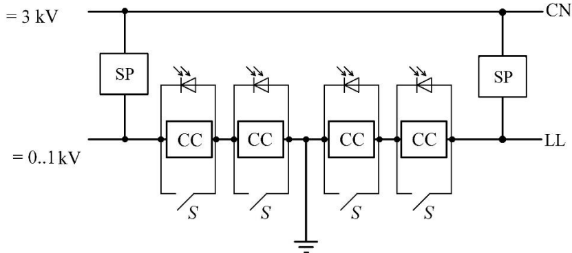
Fig. 2. Structure of the connection of distributed solar electricity generators: CN - contact network; LL - longitudinal line DC; CC - to coordinate converters; SP - traction network supply points; S - shunt keys
