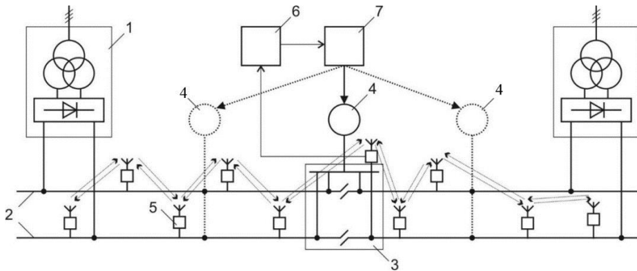
Fig. 5. The scheme of quality control voltage electrified railway section: 1 - traction substation; 2 - contact network; 3 - sectioning post; 4 - supply points; 5 - voltage measuring device with wireless data transmission; 6 - decoding unit data; 7 - control system
